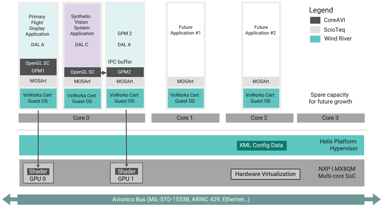
Figure 12. ScioTeq display platform architecture with example configuration
